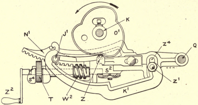
Fig. 215. Combination Builder.
